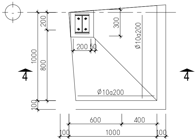
MÓNG M-4 TL 1/25
